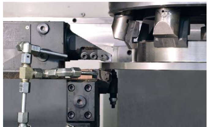
Lift-off slide in turret
