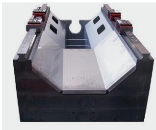
Thermo-symmetrical construction
