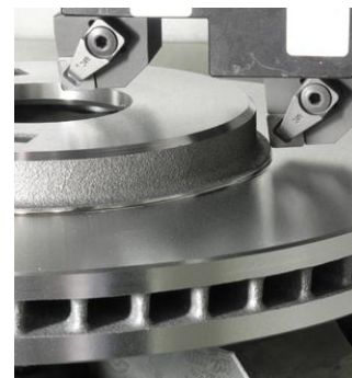
Step 4: Machine 2nd side
