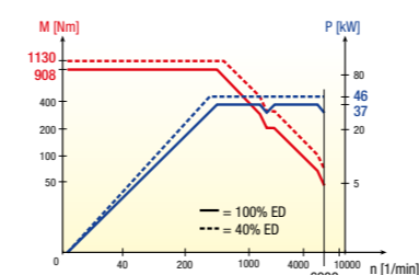
Geared spindle with 100 mm bearing diameter for NBH 630 / 800 / 1000 / 1200
