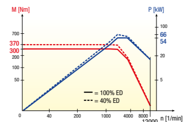
Motor spindle with 100 mm bearing diameter for NBH 6 / 6+ / 630 / 800 / 1000
