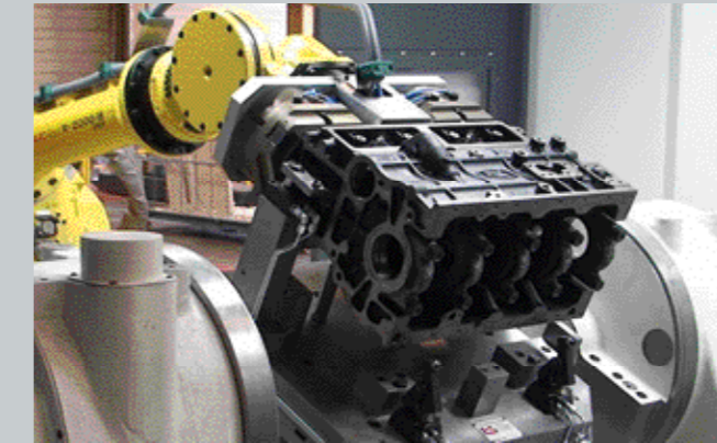
Direct loading of fixture on tilting/rotary table by means of 6-axis robot
